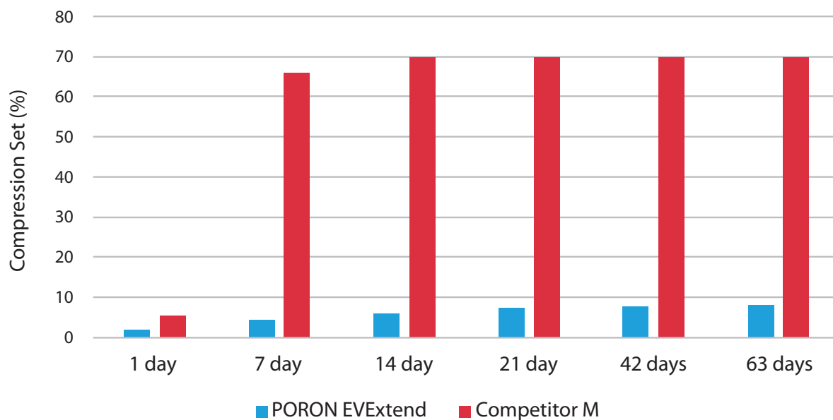
C-Set 70% 70°C
