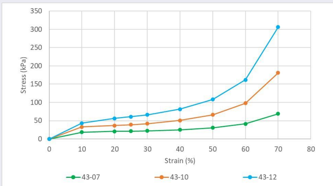
Graph 1: Compression Force Deflection Full Range (ASTM D1056)
