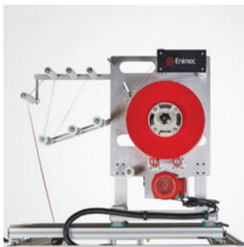
Tape spool unwinder for tear tape and other tapes in spool form
