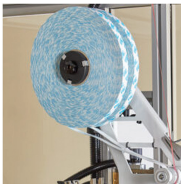
Split spindle for applying two rolls of tape on the same applicator
